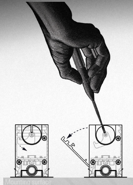
The catches at both ends of the luminaire can be turned using a flat-head screwdriver. This rotates the internal cam latches - releasing the side panel, which is then able to hinge open.
