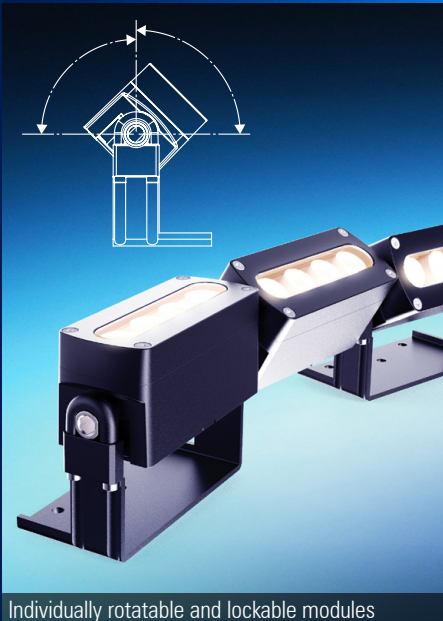
Individually rotatable and lockable modules
