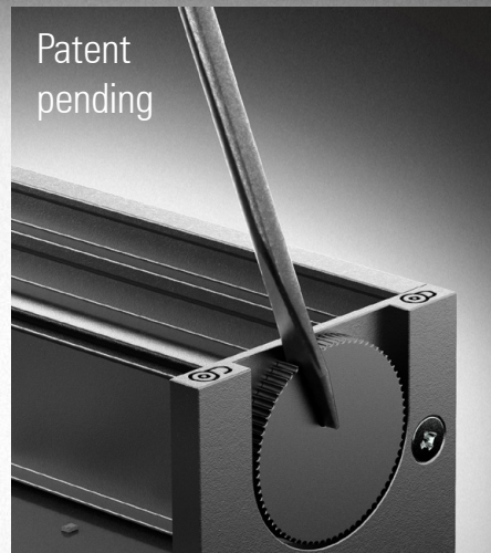
The catches at both ends of the luminaire can be turned using a flat-head screwdriver. This rotates the internal cam latches - releasing the side panel, which is then able to hinge open.
