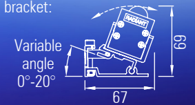
Adjustable angle bracket:
